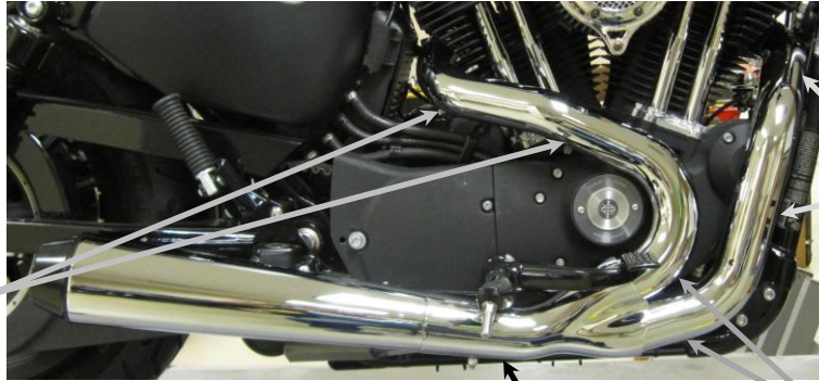
FIGURE 4 COLLECTOR HEATSHIELD
